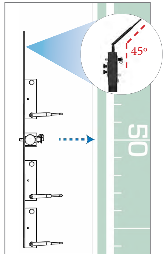
Figure 121: Top View of RT Bracket and Antenna Direction
