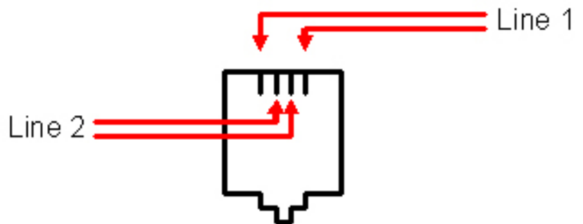
Figure 137: RJ-14 Wiring
