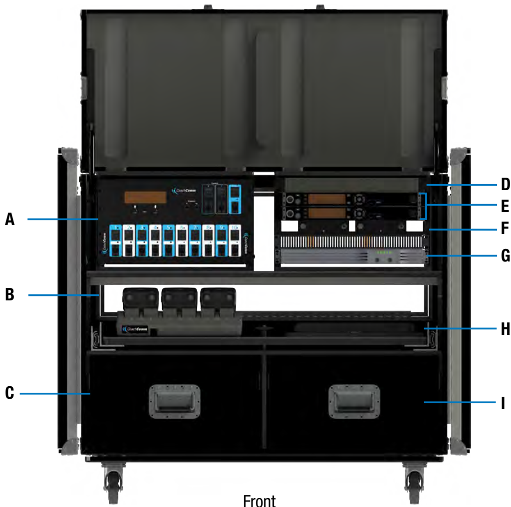
Figure 144: Wireless Press Box Unit (WPB2) Front View
