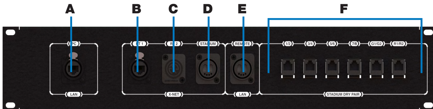
Figure 141: Wireless Press Box (WPB1) Rear Patch Panel
