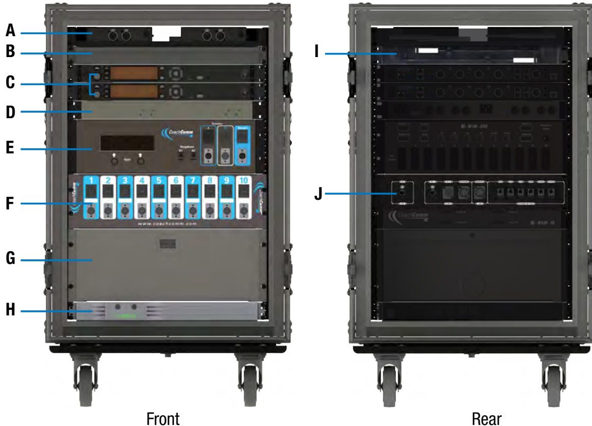
Figure 140: Wireless Press Box Unit (WPB1) Overview
