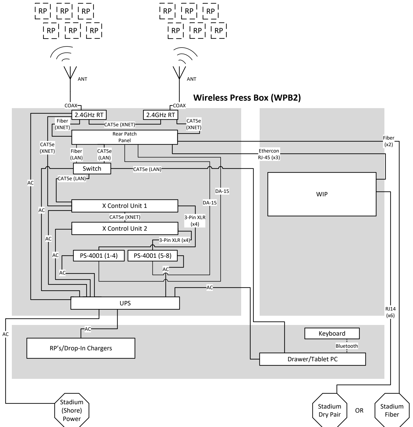
Figure 143: Wireless Press Box Unit (WPB2) Block Diagram
