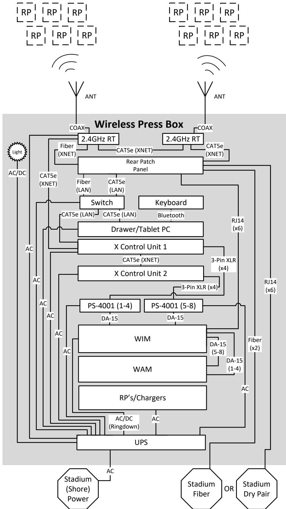
Figure 139: Wireless Press Box Unit (WPB1) Block Diagram
