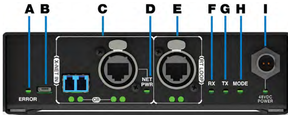
Figure 45: Radio Transceiver Bottom View
