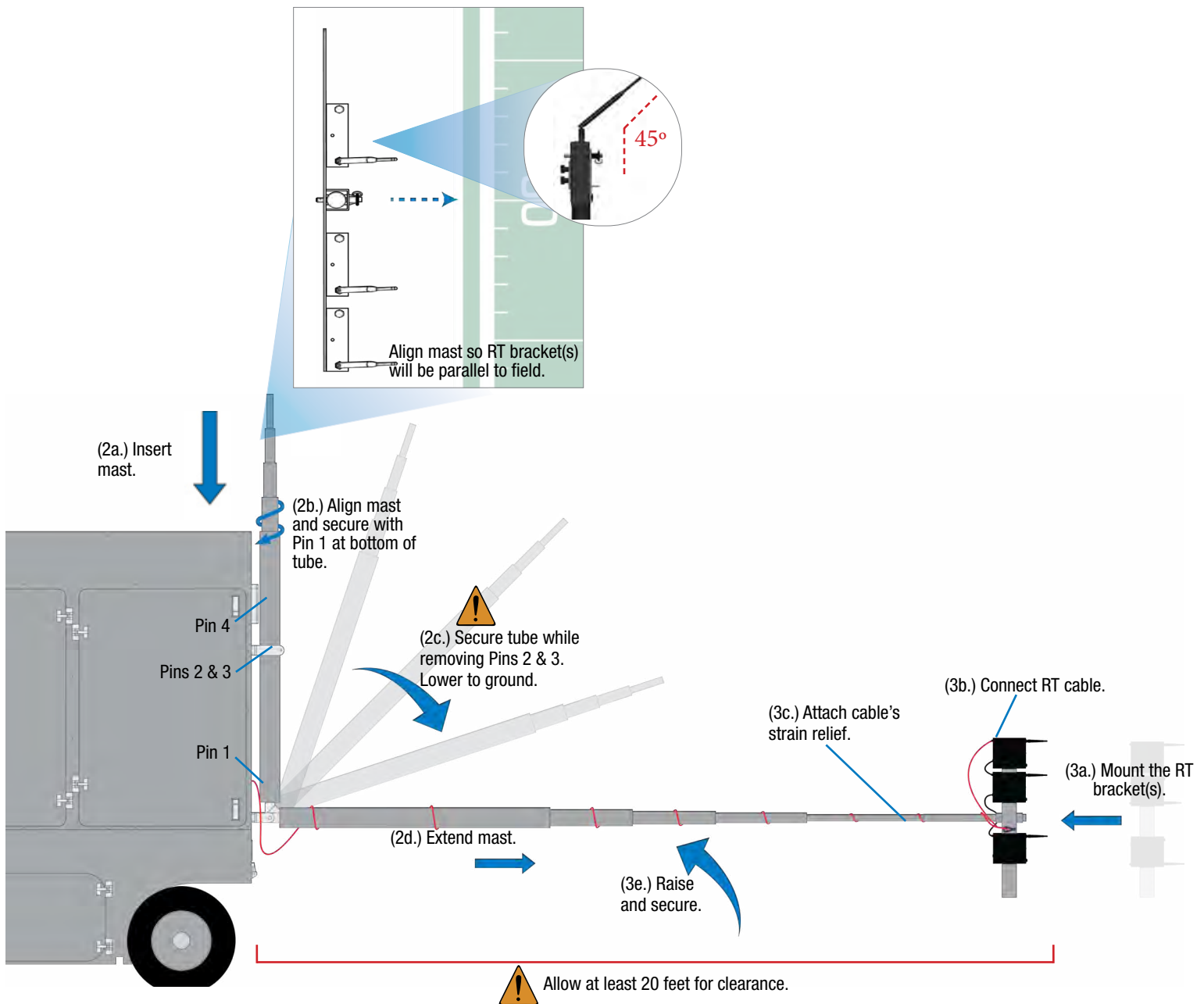
Figure 13: Sideline Cart RT Mast Setup
