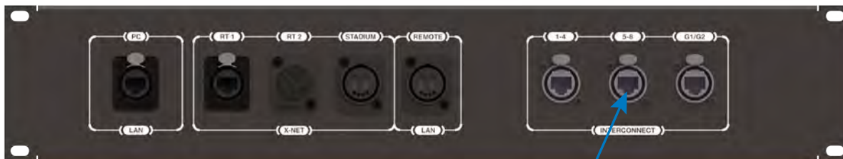
Wireless Press Box Unit (WPB2) Rear Panel
