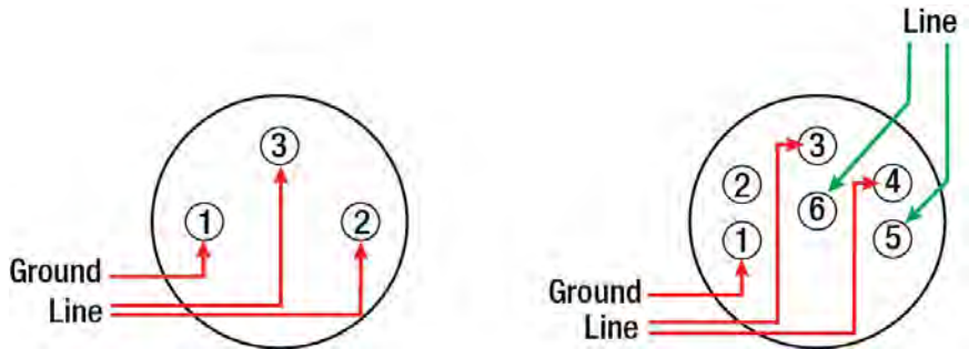
Figure 136: XLR Terminations
