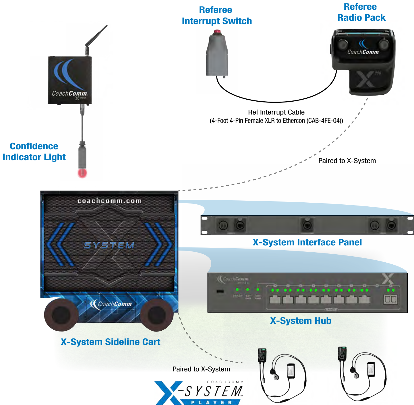
Figure 148: CoachComm X-System Player Block Diagram (Single Wirelsss Referee Interrupt Configuration)
